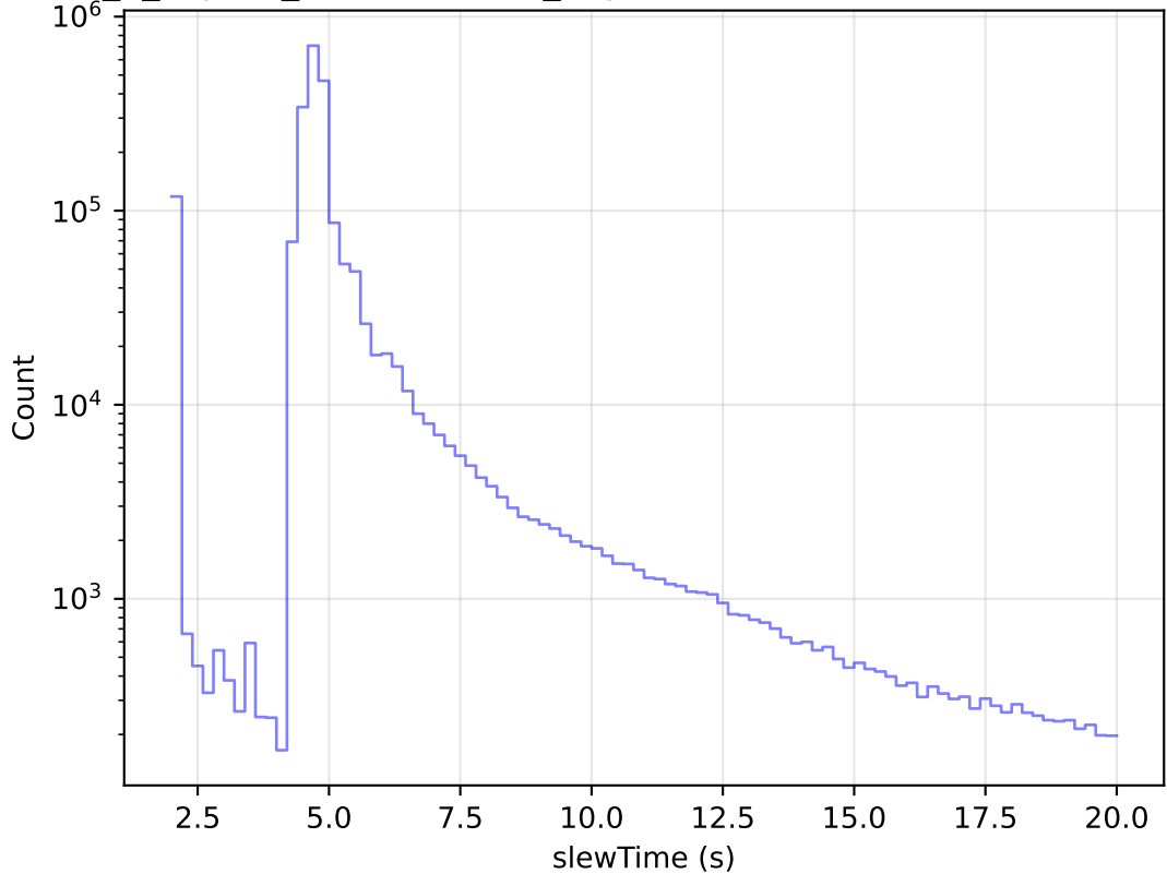
internal_u_expt27_nscale1.0v3.4_10yrs All visits: Zoom Slew Time Histogram
