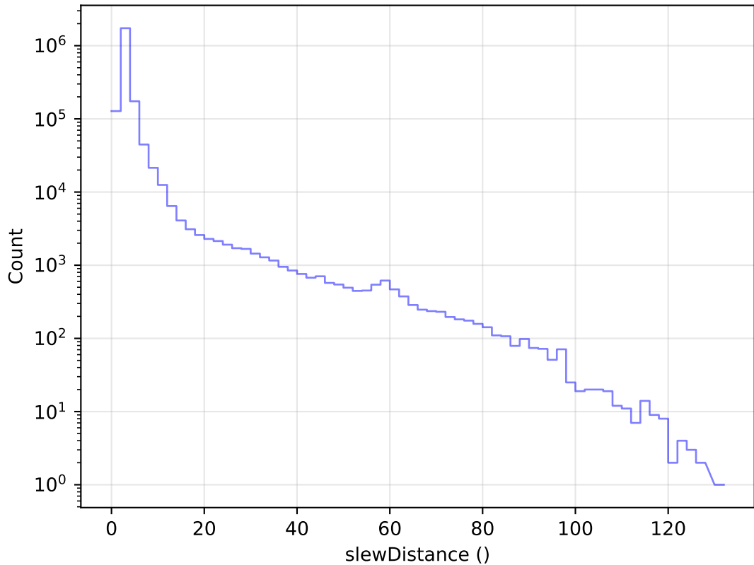
internal_u_expt27_nscale1.0v3.4_10yrs All visits: Slew Distance Histogram
