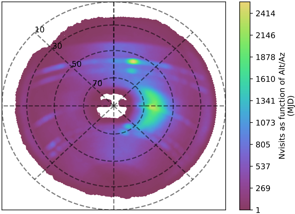
internal_u_expt27_nscale1.0v3.4_10yrs z band: Nvisits as function of Alt/Az
