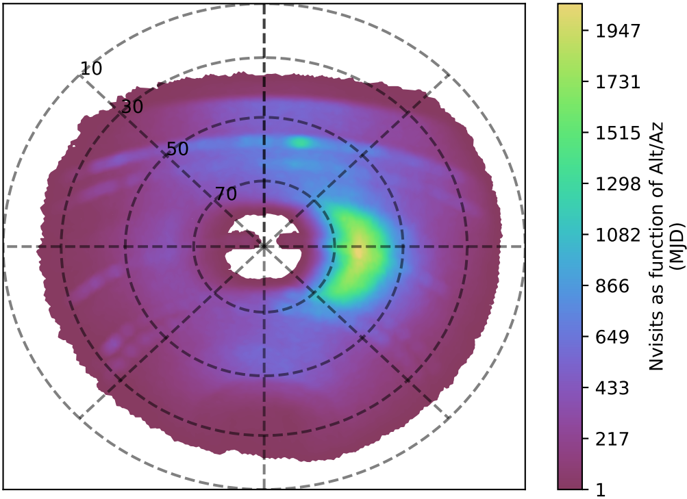
internal_u_expt27_nscale1.0v3.4_10yrs y band: Nvisits as function of Alt/Az
