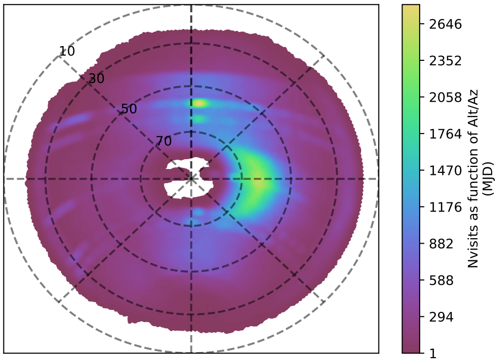
internal_u_expt27_nscale1.0v3.4_10yrs i band: Nvisits as function of Alt/Az
