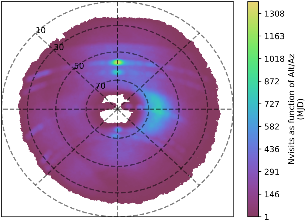
internal_u_expt27_nscale1.0v3.4_10yrs g band: Nvisits as function of Alt/Az
