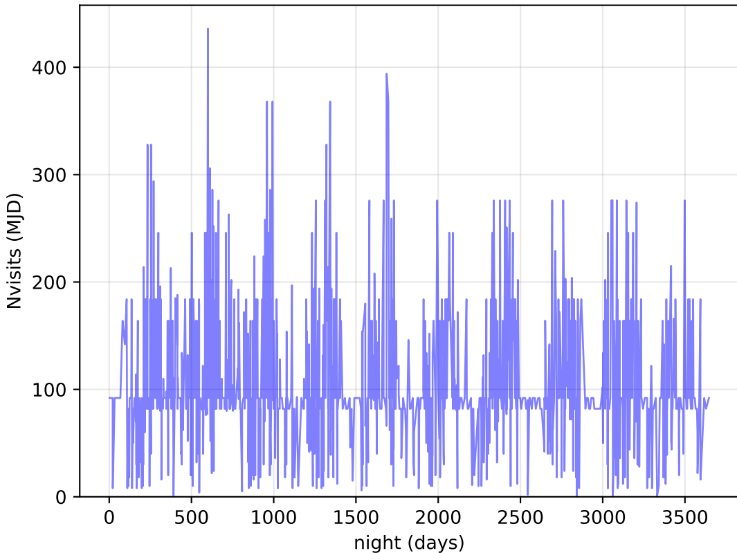
internal_u_expt27_nscale1.0v3.4_10yrs DDF: Nvisits
