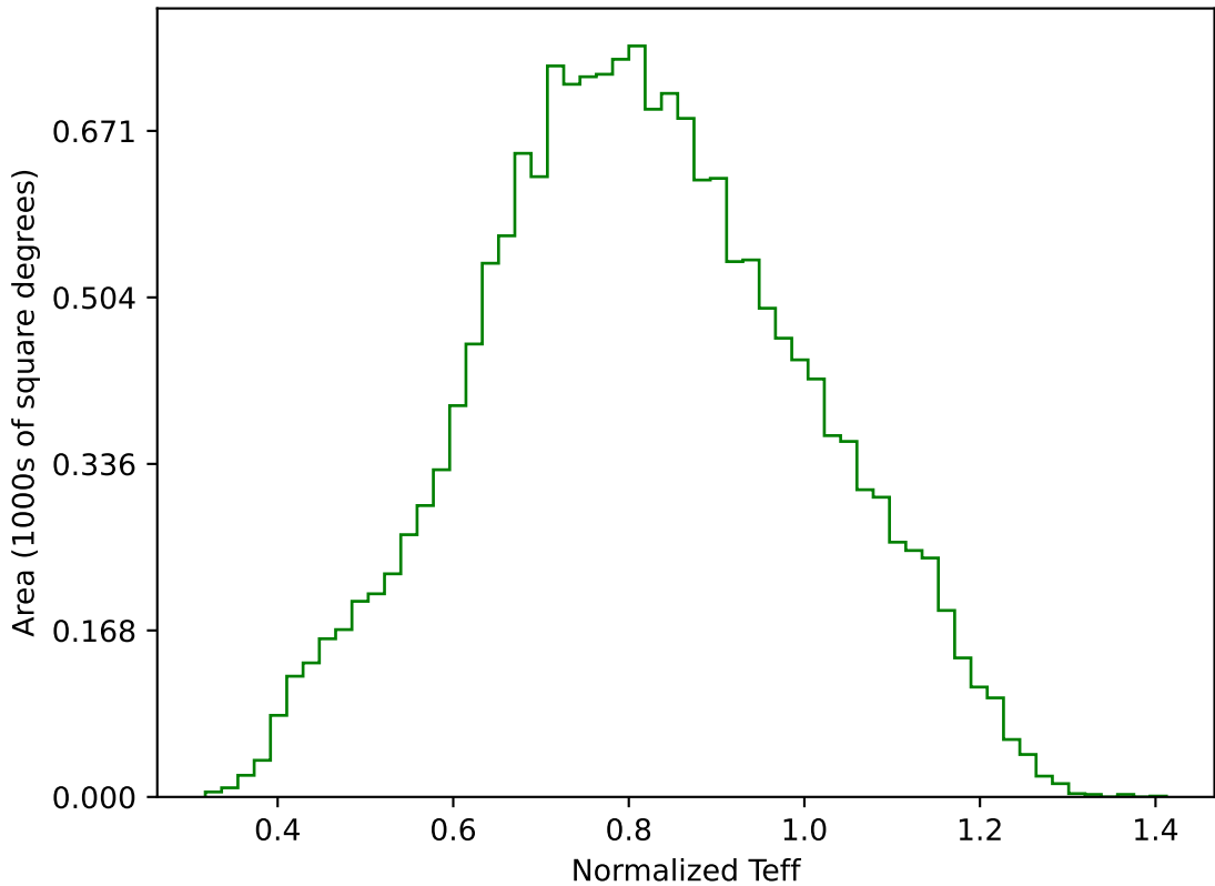
internal_u_expt27_nscale1.0v3.4_10yrs WFD g band: Normalized Teff
