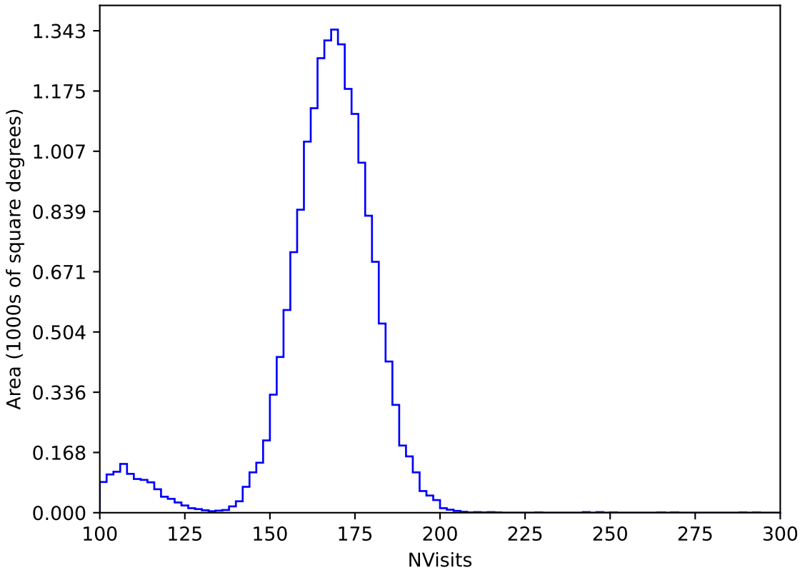
internal_u_expt27_nscale1.0v3.4_10yrs WFD y band: NVisits
