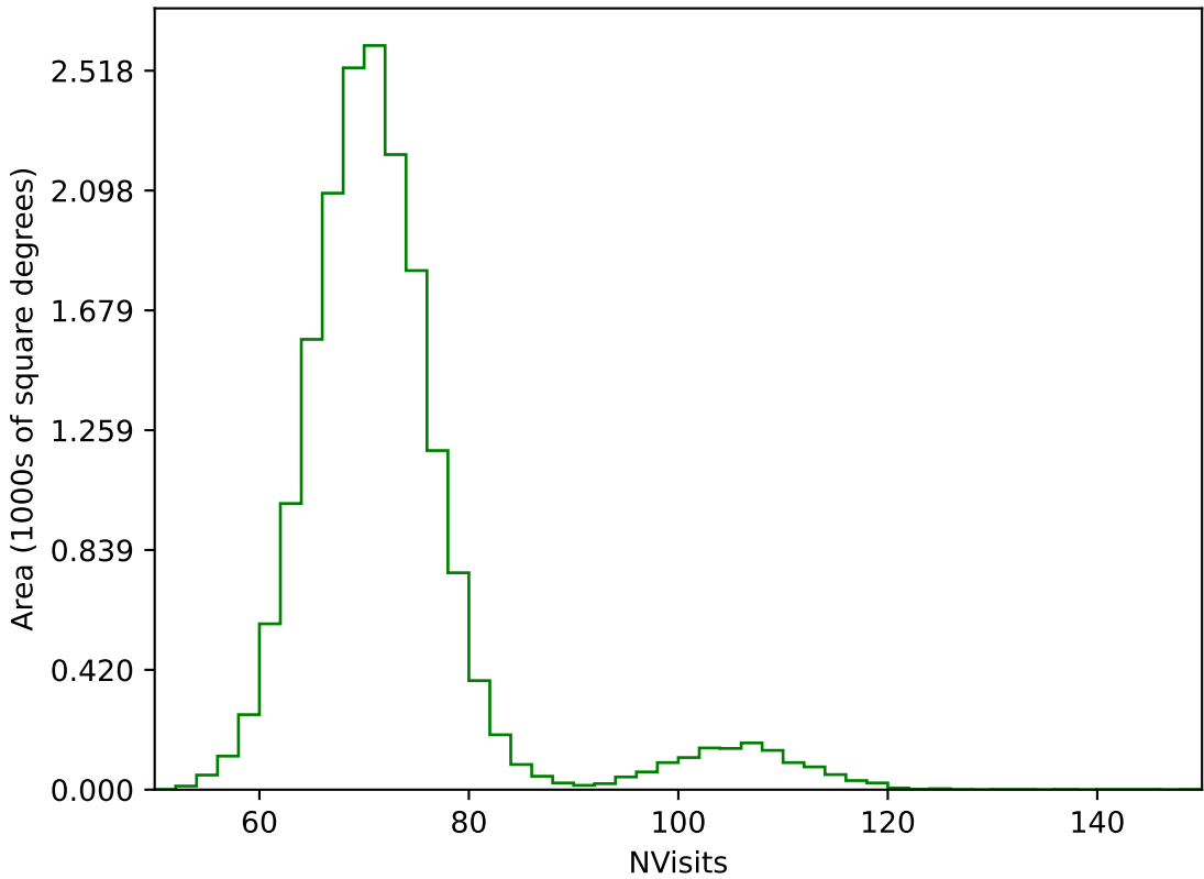
internal_u_expt27_nscale1.0v3.4_10yrs WFD g band: NVisits
