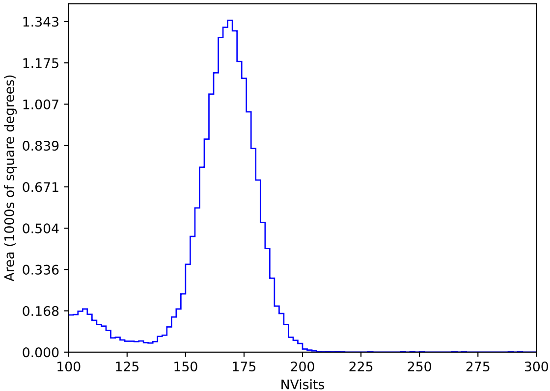
internal_u_expt27_nscale1.0v3.4_10yrs All sky y band: NVisits
