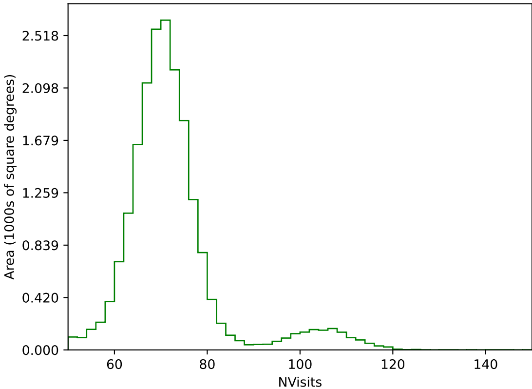
internal_u_expt27_nscale1.0v3.4_10yrs All sky g band: NVisits
