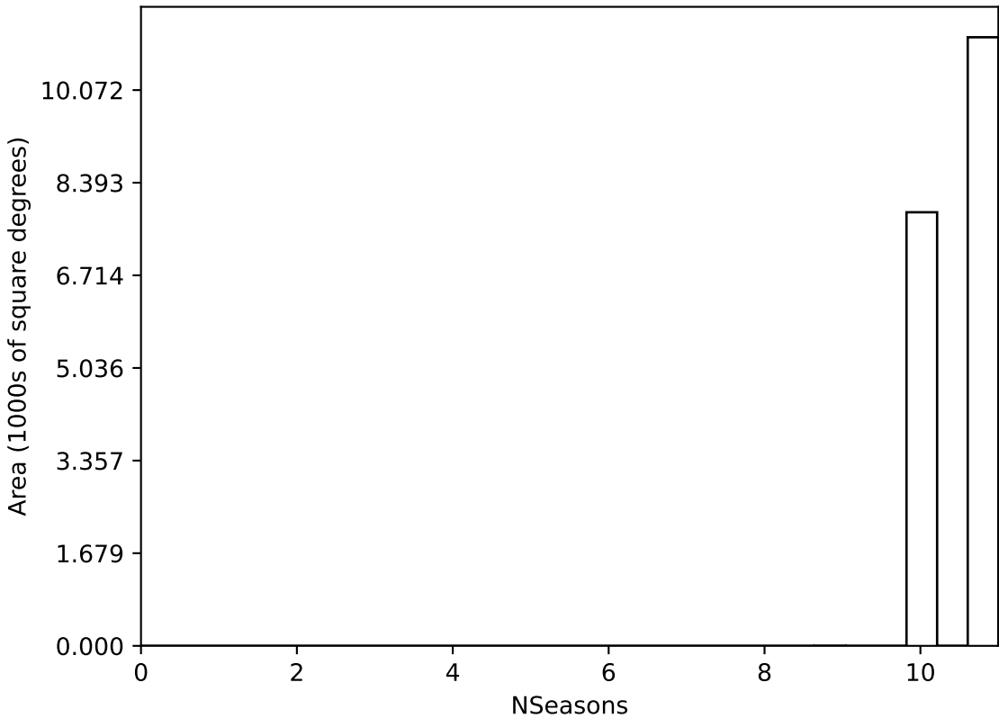
internal_u_expt27_nscale1.0v3.4_10yrs WFD all bands: NSeasons
