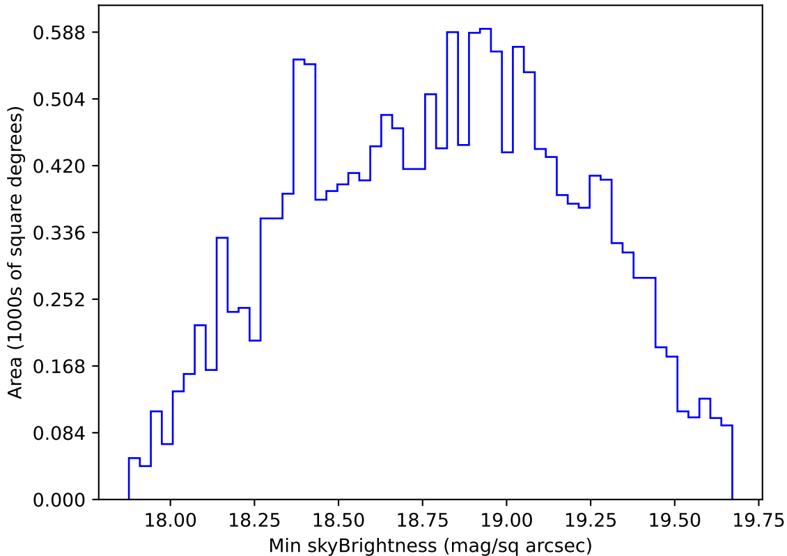
internal_u_expt27_nscale1.0v3.4_10yrs WFD r band: Min skyBrightness
