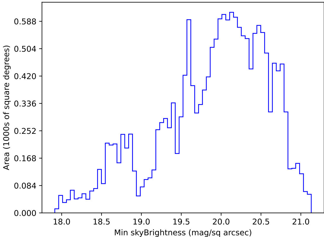
internal_u_expt27_nscale1.0v3.4_10yrs WFD g band: Min skyBrightness
