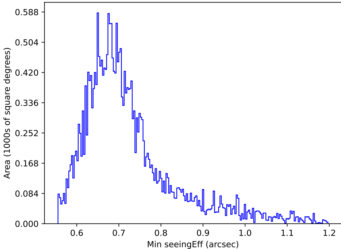
internal_u_expt27_nscale1.0v3.4_10yrs Yr 1 z band: Min seeingEff
