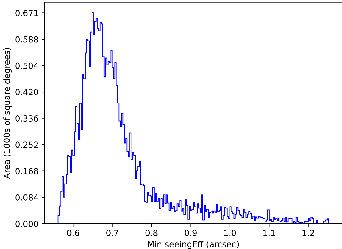
internal_u_expt27_nscale1.0v3.4_10yrs Yr 1 i band: Min seeingEff
