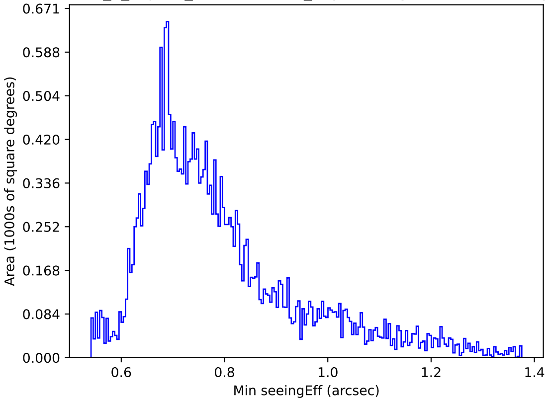
internal_u_expt27_nscale1.0v3.4_10yrs Yr 1 g band: Min seeingEff
