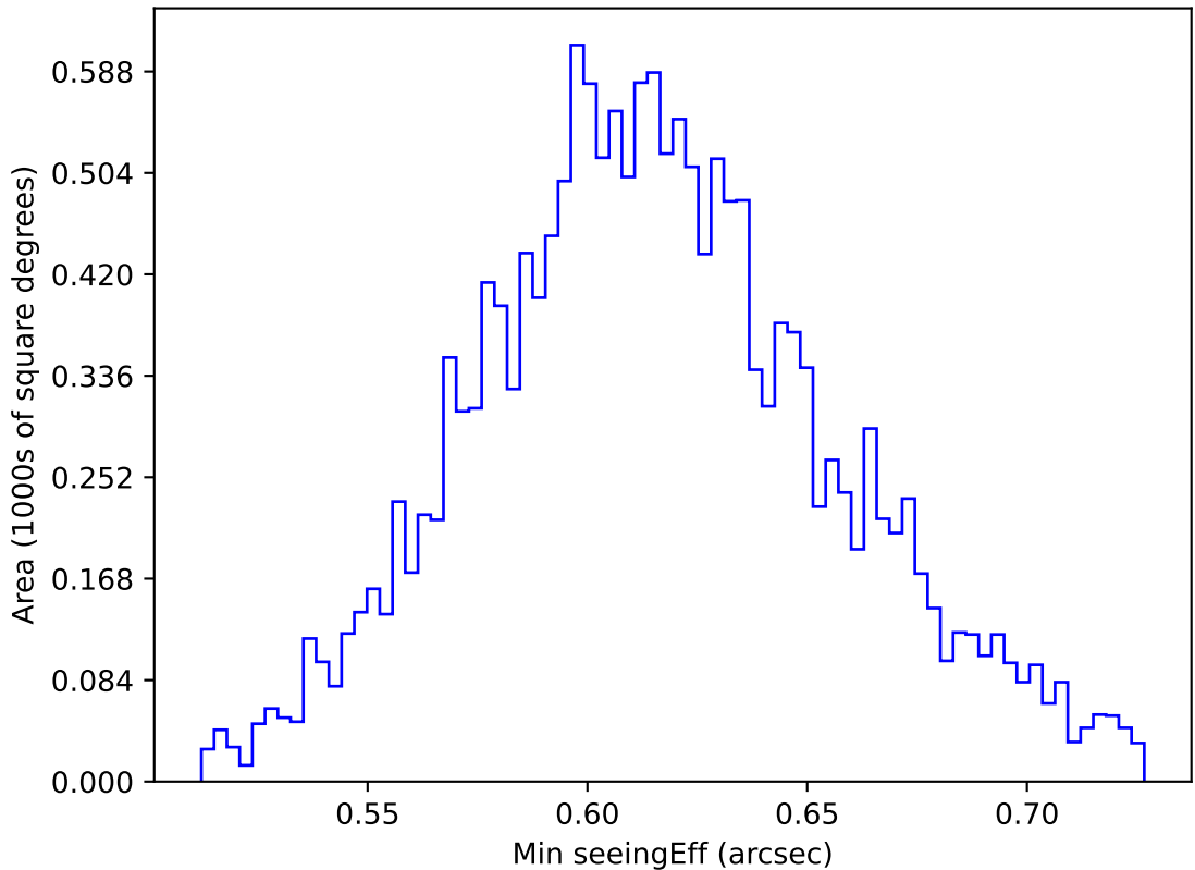
internal_u_expt27_nscale1.0v3.4_10yrs WFD z band: Min seeingEff
