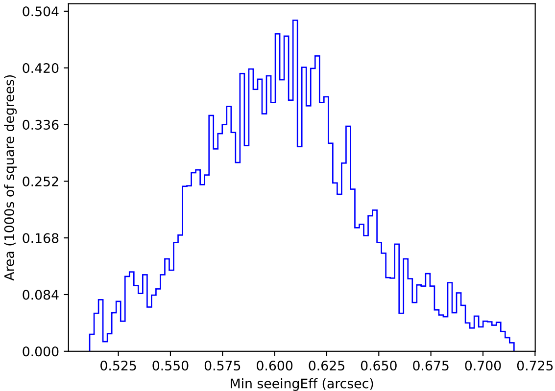
internal_u_expt27_nscale1.0v3.4_10yrs WFD i band: Min seeingEff
