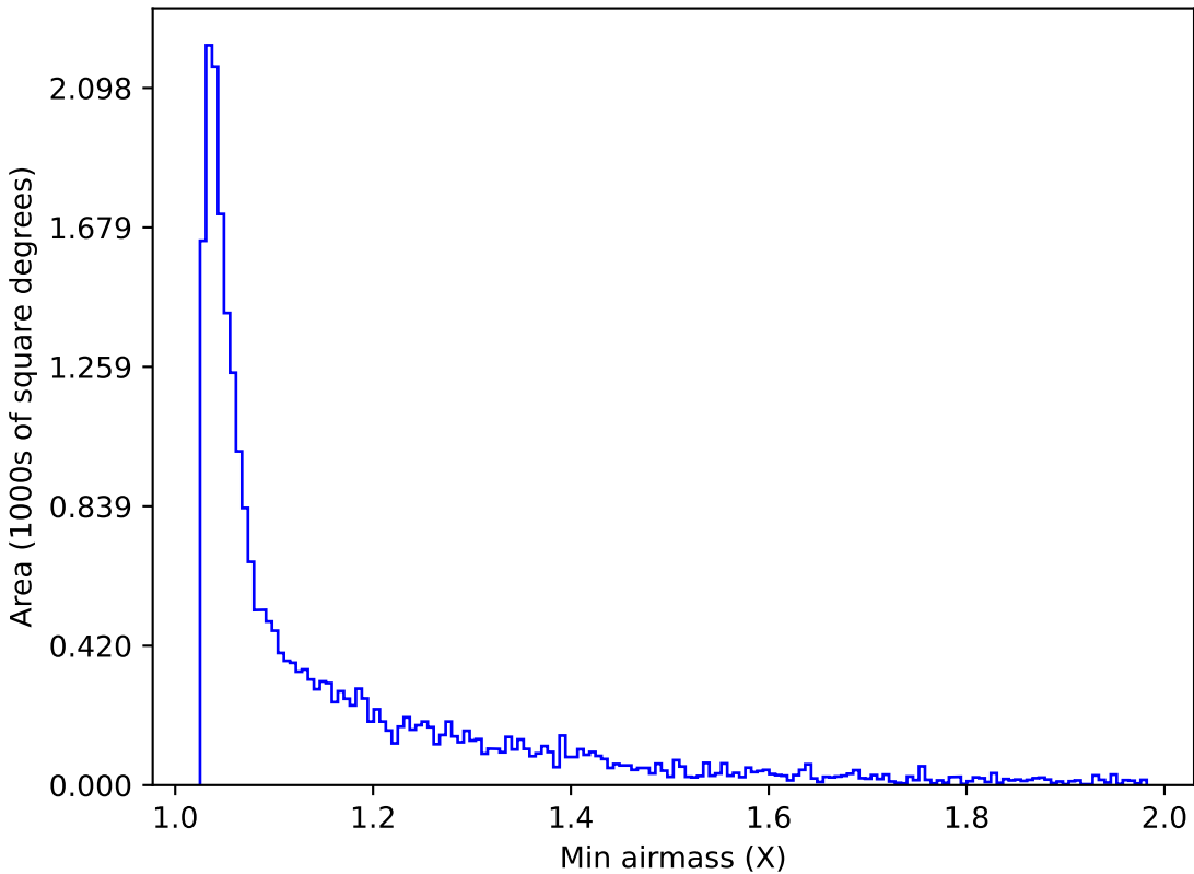
internal_u_expt27_nscale1.0v3.4_10yrs Yr 1 z band: Min airmass
