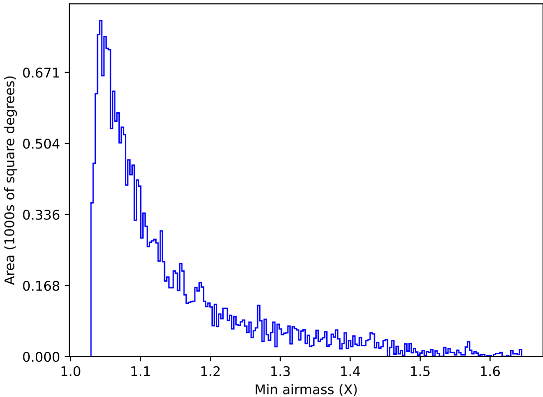
internal_u_expt27_nscale1.0v3.4_10yrs Yr 1 u band: Min airmass
