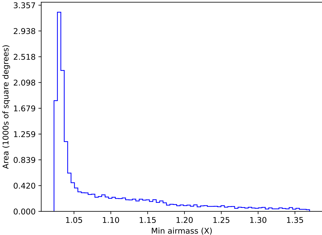
internal_u_expt27_nscale1.0v3.4_10yrs WFD y band: Min airmass
