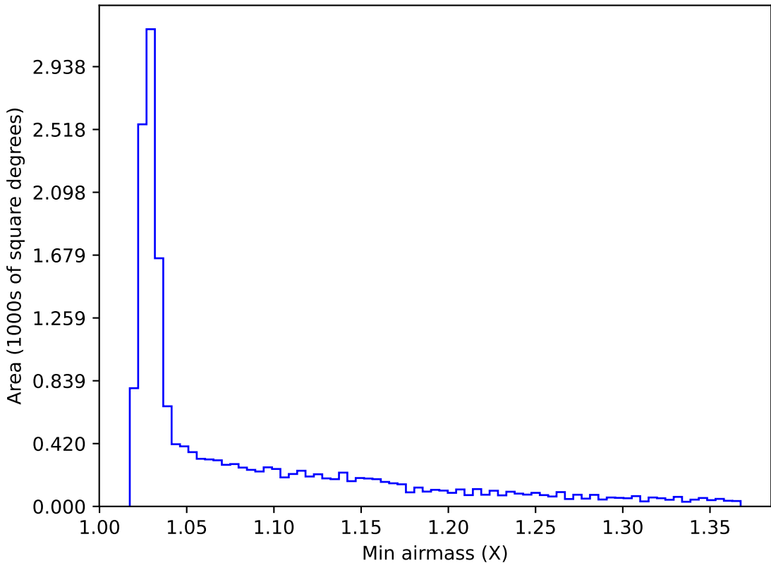
internal_u_expt27_nscale1.0v3.4_10yrs WFD i band: Min airmass
