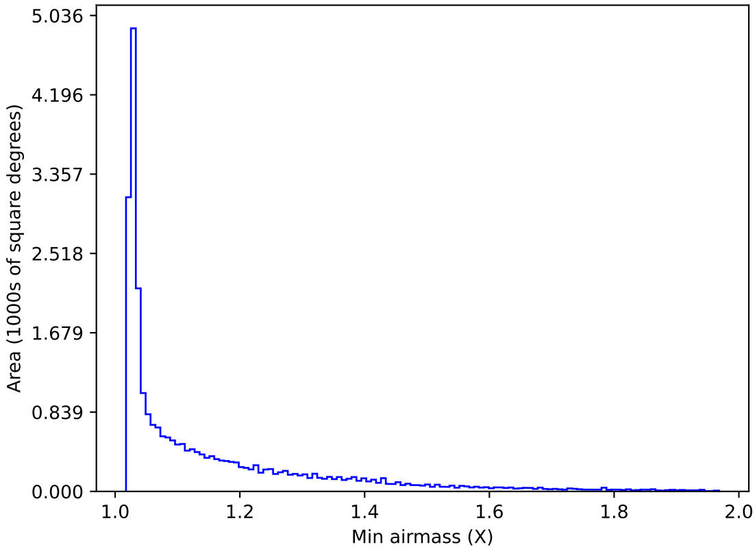
internal_u_expt27_nscale1.0v3.4_10yrs All sky r band: Min airmass
