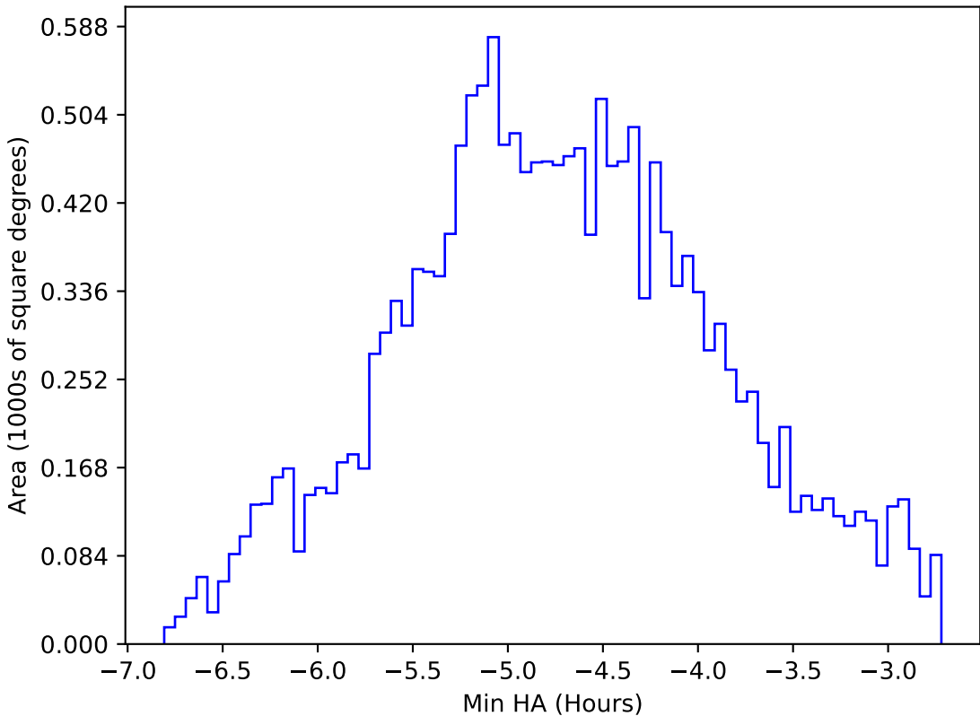
internal_u_expt27_nscale1.0v3.4_10yrs WFD all bands: Min HA
