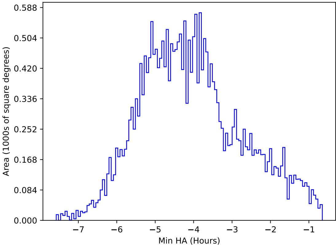
internal_u_expt27_nscale1.0v3.4_10yrs All sky z band: Min HA
