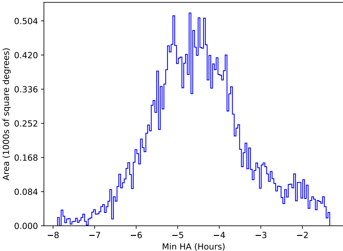
internal_u_expt27_nscale1.0v3.4_10yrs All sky all bands: Min HA
