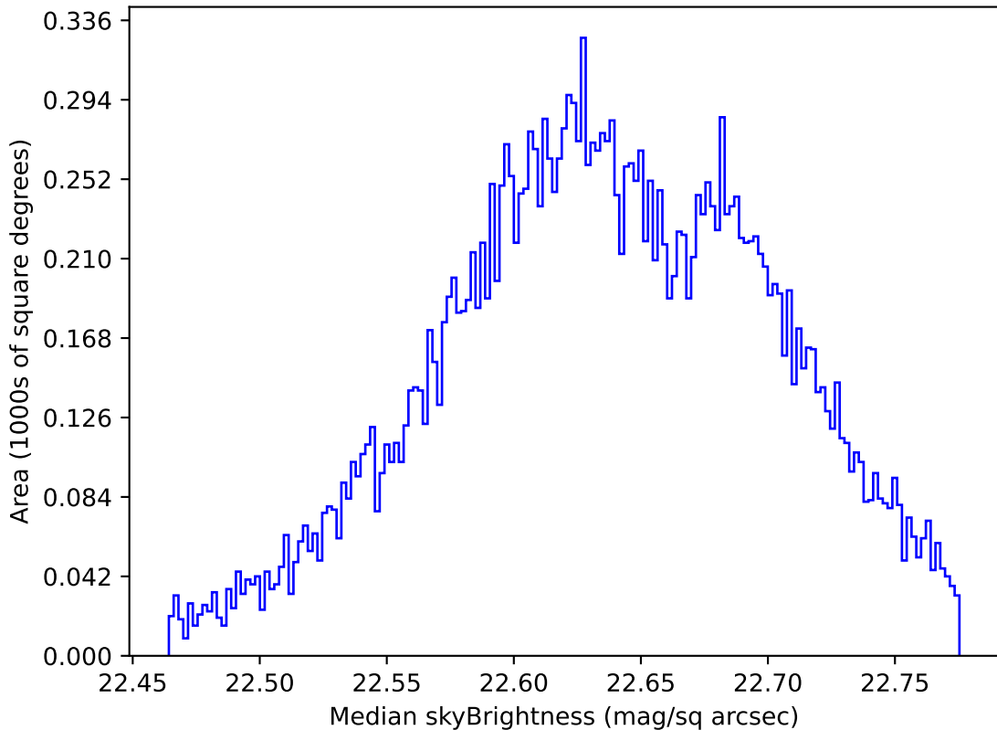
internal_u_expt27_nscale1.0v3.4_10yrs Yr 1 u band: Median skyBrightness
