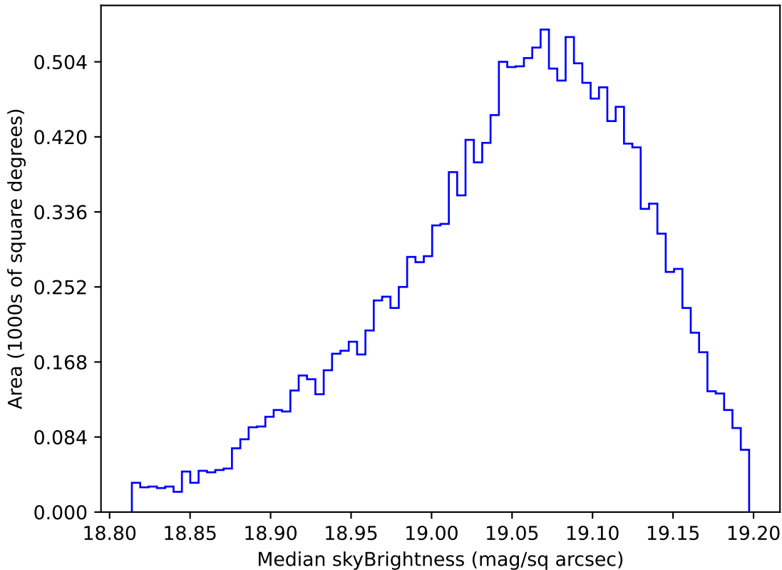
internal_u_expt27_nscale1.0v3.4_10yrs WFD z band: Median skyBrightness
