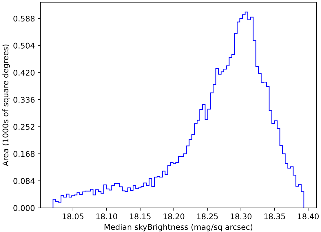
internal_u_expt27_nscale1.0v3.4_10yrs WFD y band: Median skyBrightness
