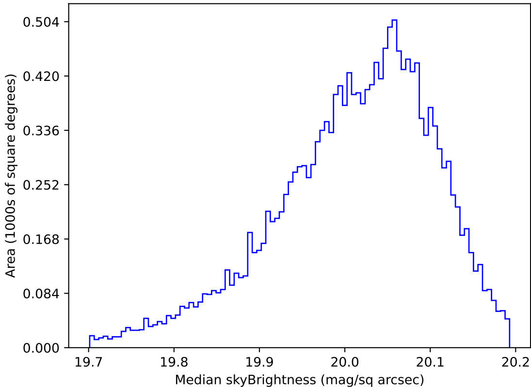
internal_u_expt27_nscale1.0v3.4_10yrs WFD i band: Median skyBrightness
