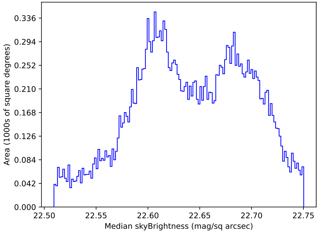
internal_u_expt27_nscale1.0v3.4_10yrs All sky u band: Median skyBrightness
