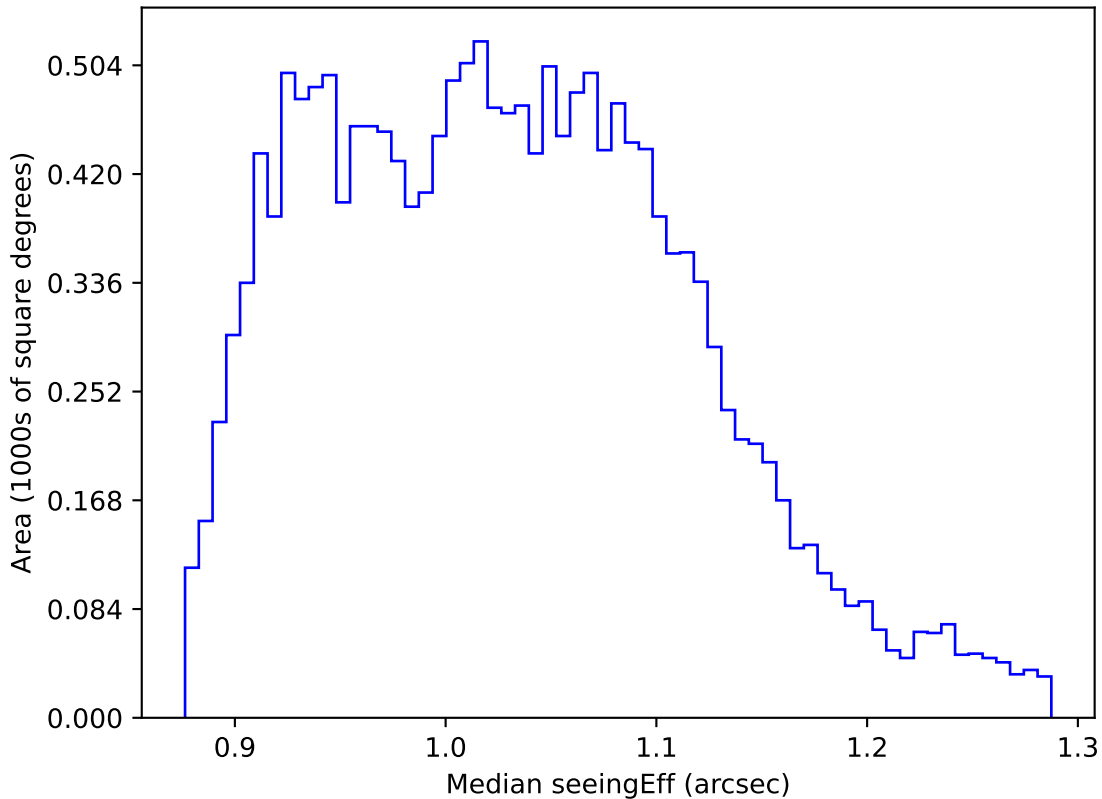
internal_u_expt27_nscale1.0v3.4_10yrs WFD r band: Median seeingEff
