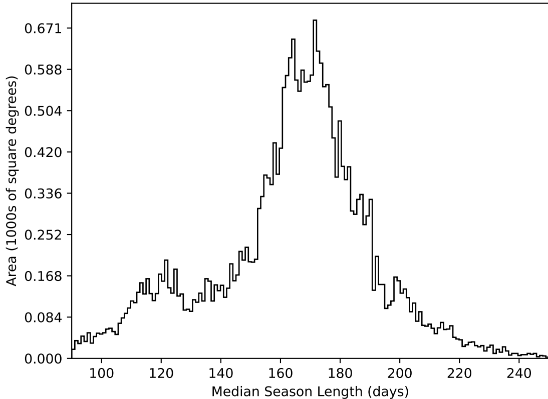
internal_u_expt27_nscale1.0v3.4_10yrs All sky all bands: Median Season Length
