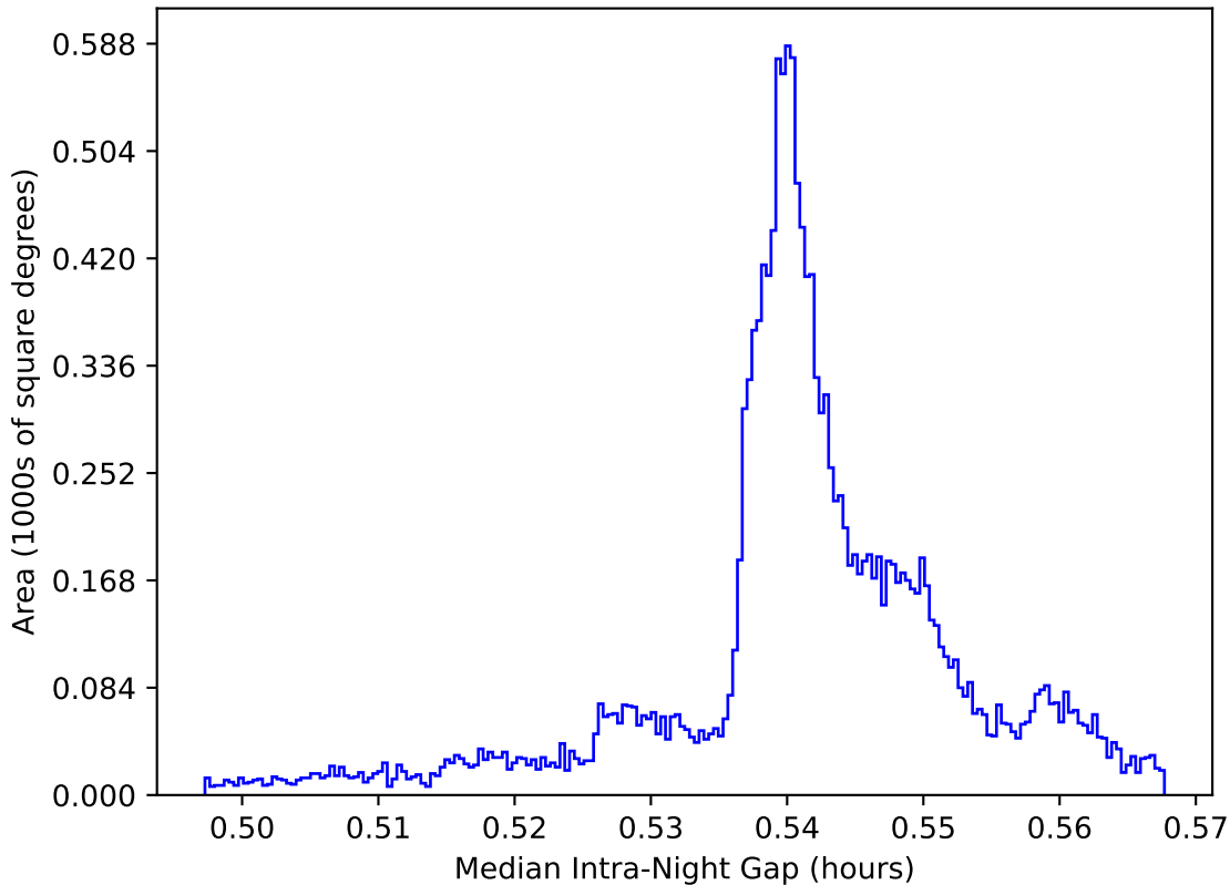
internal_u_expt27_nscale1.0v3.4_10yrs WFD: Median Intra-Night Gap
