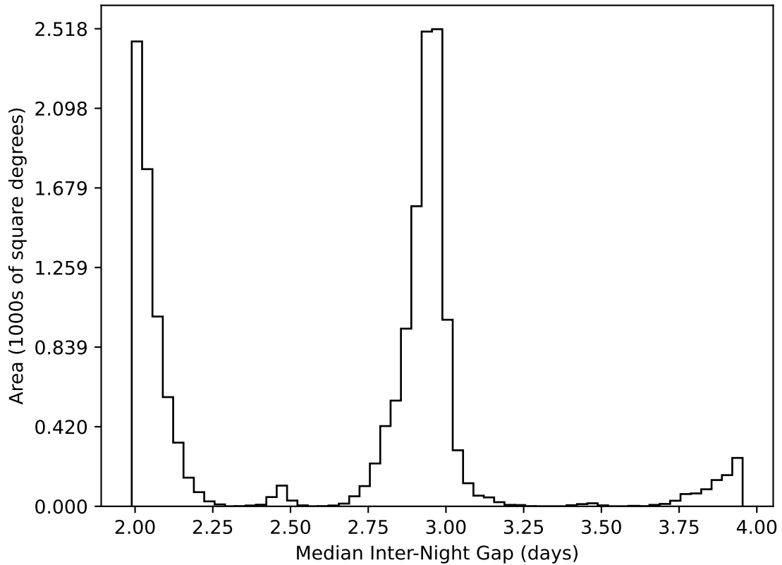
internal_u_expt27_nscale1.0v3.4_10yrs WFD all bands: Median Inter-Night Gap
