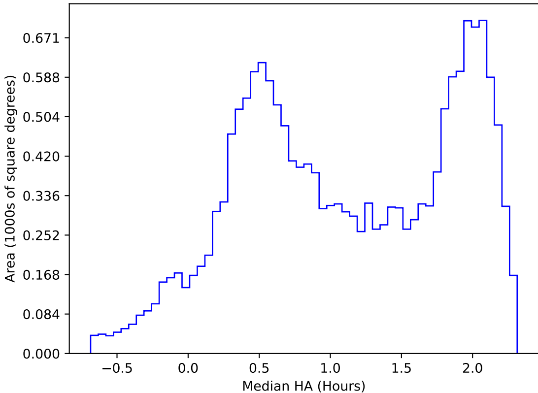
internal_u_expt27_nscale1.0v3.4_10yrs WFD z band: Median HA
