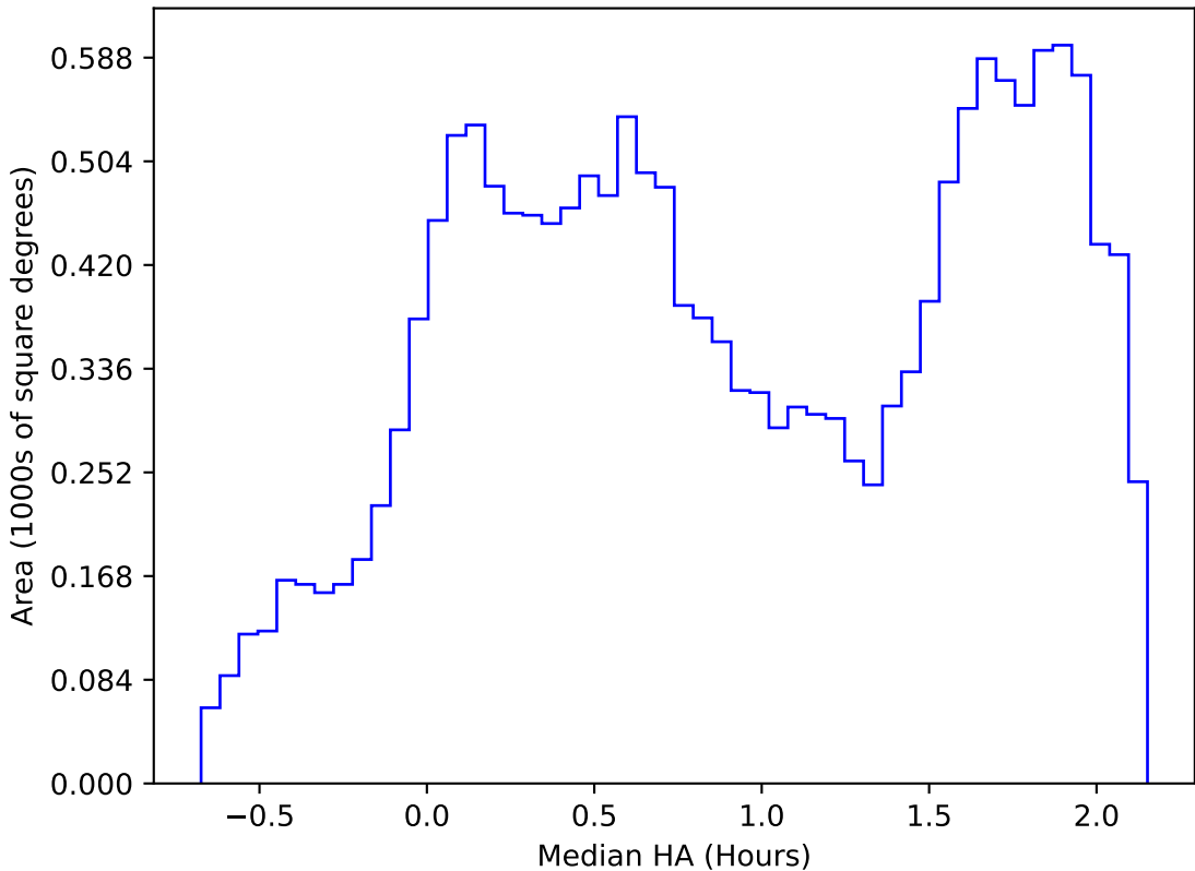
internal_u_expt27_nscale1.0v3.4_10yrs WFD r band: Median HA
