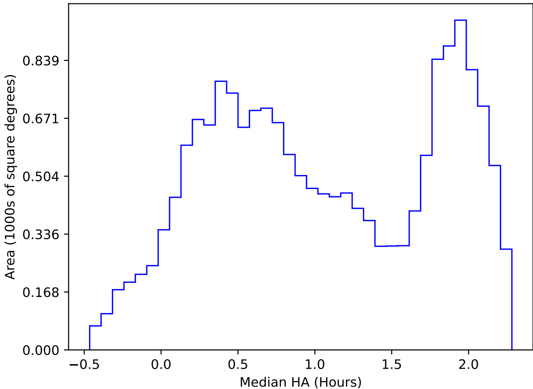
internal_u_expt27_nscale1.0v3.4_10yrs WFD i band: Median HA
