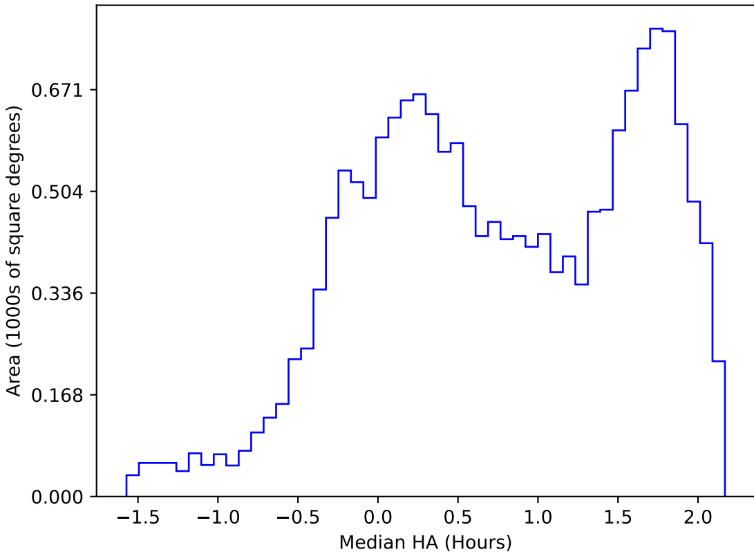
internal_u_expt27_nscale1.0v3.4_10yrs WFD g band: Median HA
