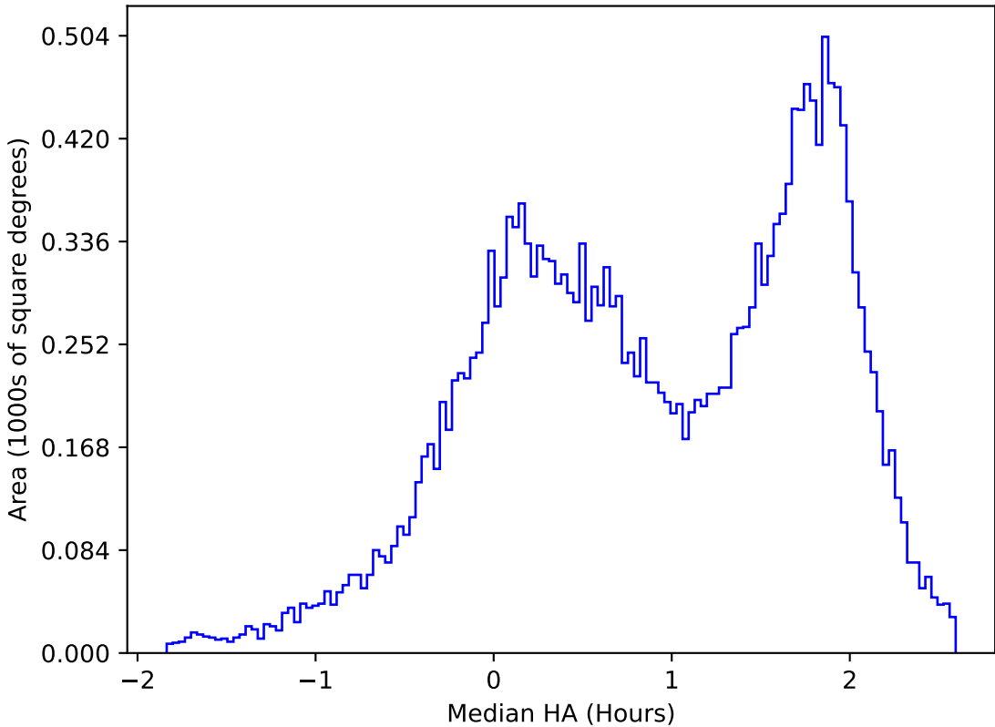
internal_u_expt27_nscale1.0v3.4_10yrs All sky u band: Median HA
