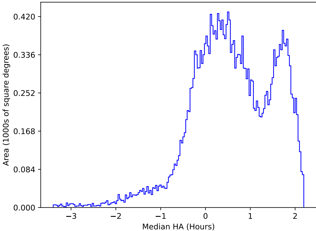
internal_u_expt27_nscale1.0v3.4_10yrs All sky g band: Median HA
