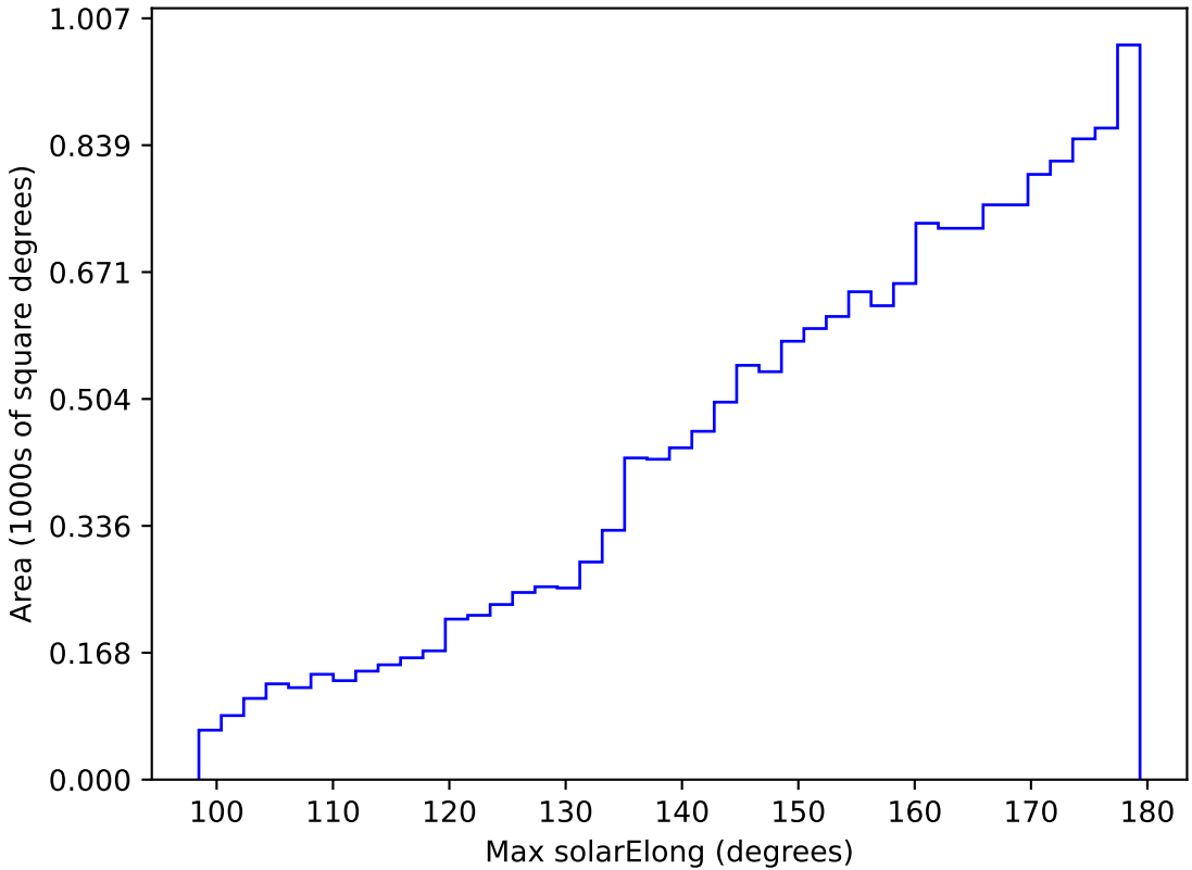
internal_u_expt27_nscale1.0v3.4_10yrs WFD y band: Max solarElong
