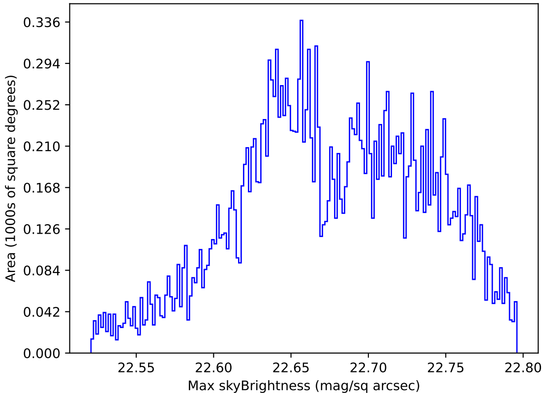
internal_u_expt27_nscale1.0v3.4_10yrs Yr 1 u band: Max skyBrightness
