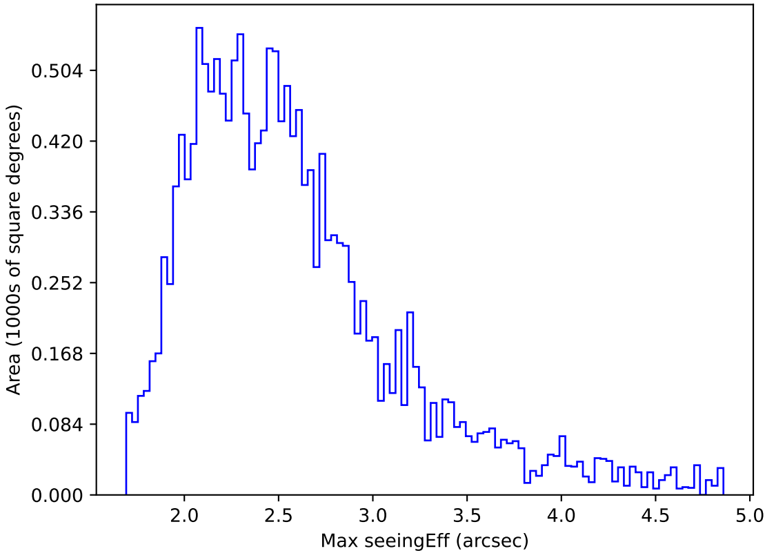
internal_u_expt27_nscale1.0v3.4_10yrs WFD z band: Max seeingEff
