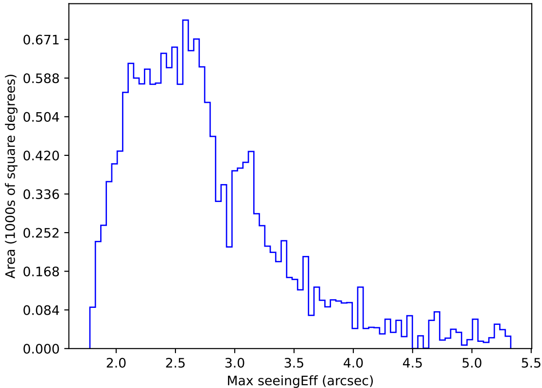
internal_u_expt27_nscale1.0v3.4_10yrs WFD i band: Max seeingEff
