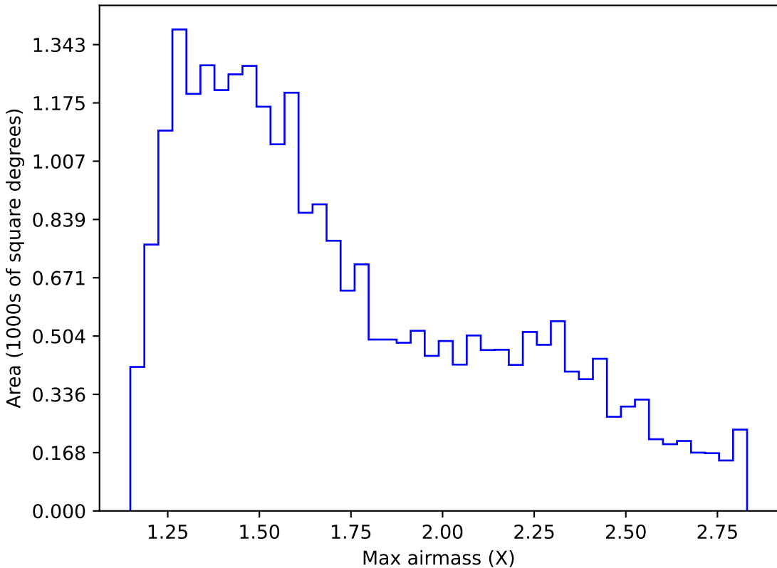
internal_u_expt27_nscale1.0v3.4_10yrs Yr 1 z band: Max airmass
