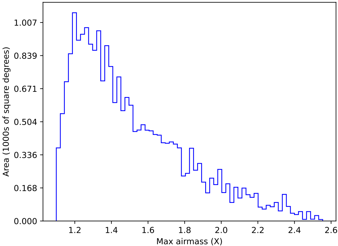
internal_u_expt27_nscale1.0v3.4_10yrs Yr 1 u band: Max airmass
