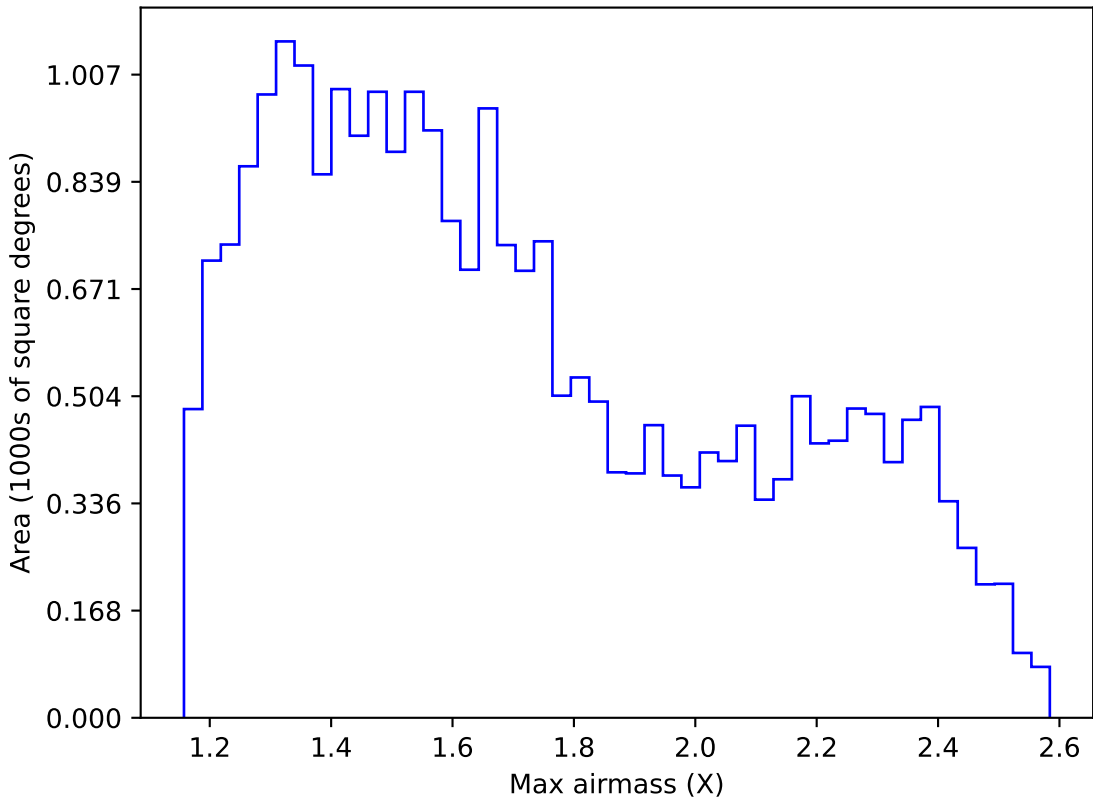
internal_u_expt27_nscale1.0v3.4_10yrs Yr 1 r band: Max airmass
